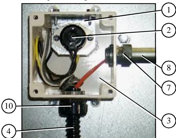
Lower plenum high limit thermostat.
